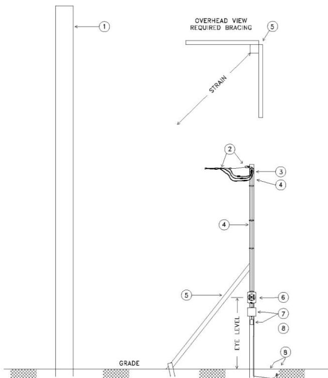
TEMPORARY OVERHEAD SERVICE CONSTRUCTION 120/240 VOLT 200 AMP SINGLE PHASE
